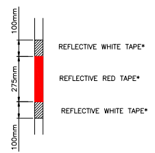
REFLECTIVE TAPE DETAIL 'A' NOT TO SCALE
