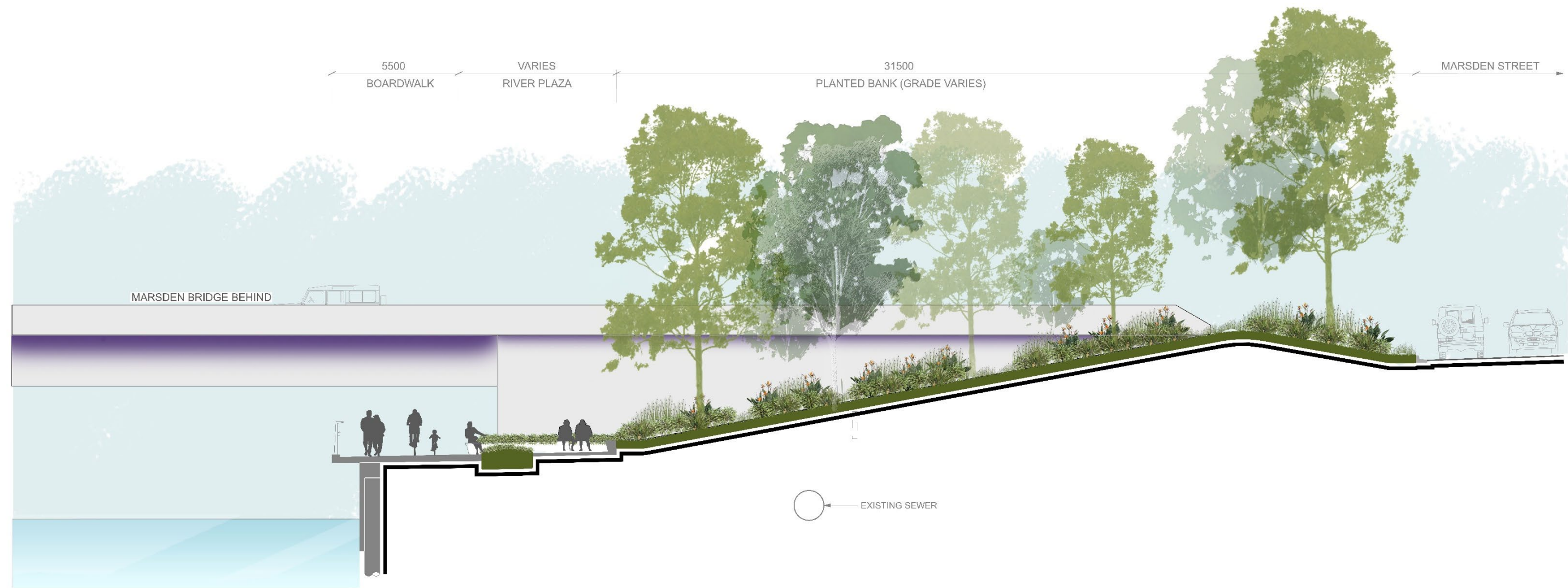
Section C – looking east showing the southern foreshore walk on approach to existing Marsden Street bridge and landscape embankment.
