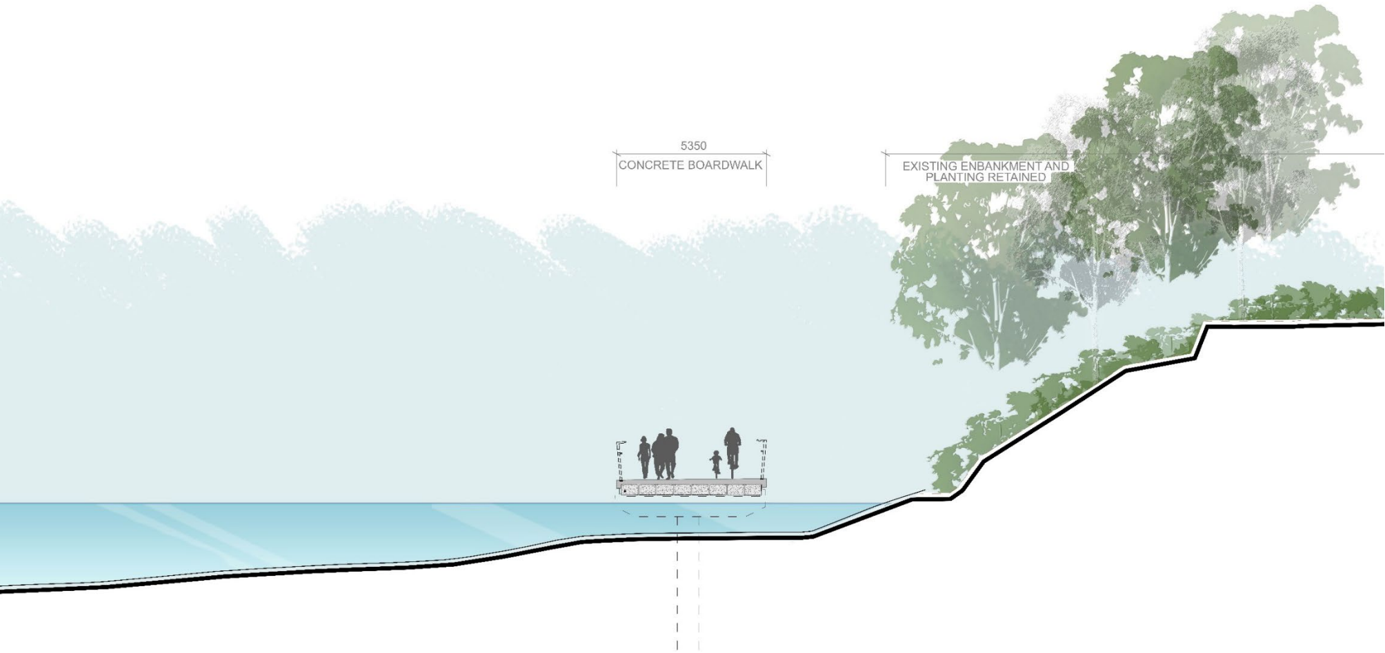
Section G – looking east showing the new boardwalk section over the river, with existing vegetated sloping embankment up to Justice Precinct
