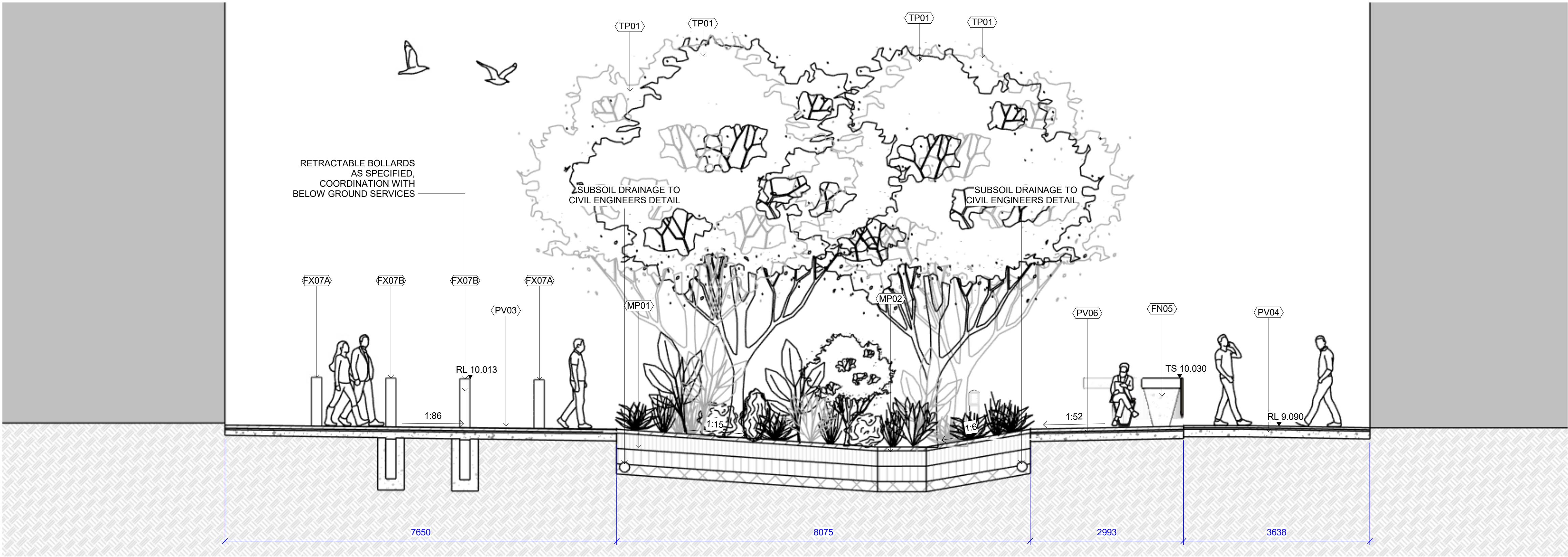
1 WSUD RAINGARDEN SECTION 3 L700 1:50
